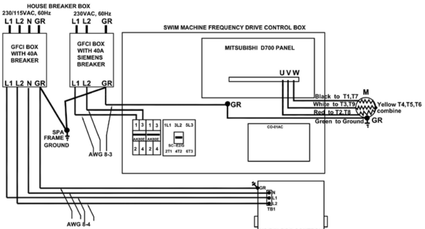
SWIMMER EDGE SE18(US, CANADA). WIRING DIAGRAM FOR TWO POWER SERVICES (40A SIEMENS GFCI, 40A GFCI).
