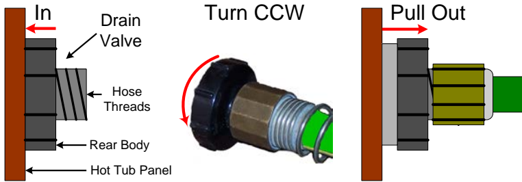
Figure 32 - Drain Operation
