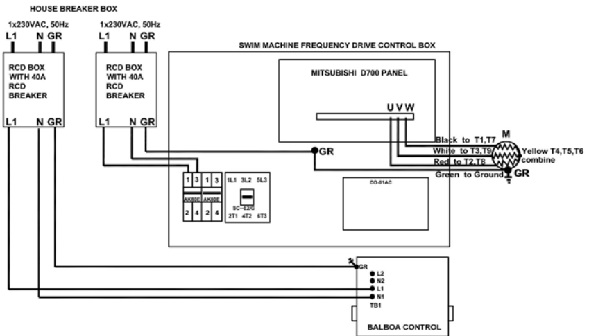
SWIMMER EDGE SE18 (EXPORT). WIRING DIAGRAM FOR TWO POWER SERVICES (2x40A RCD).
