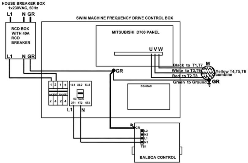
SWIMMER EDGE SE18 (EXPORT). WIRING DIAGRAM FOR ONE POWER SERVICE. (40A RCD).
