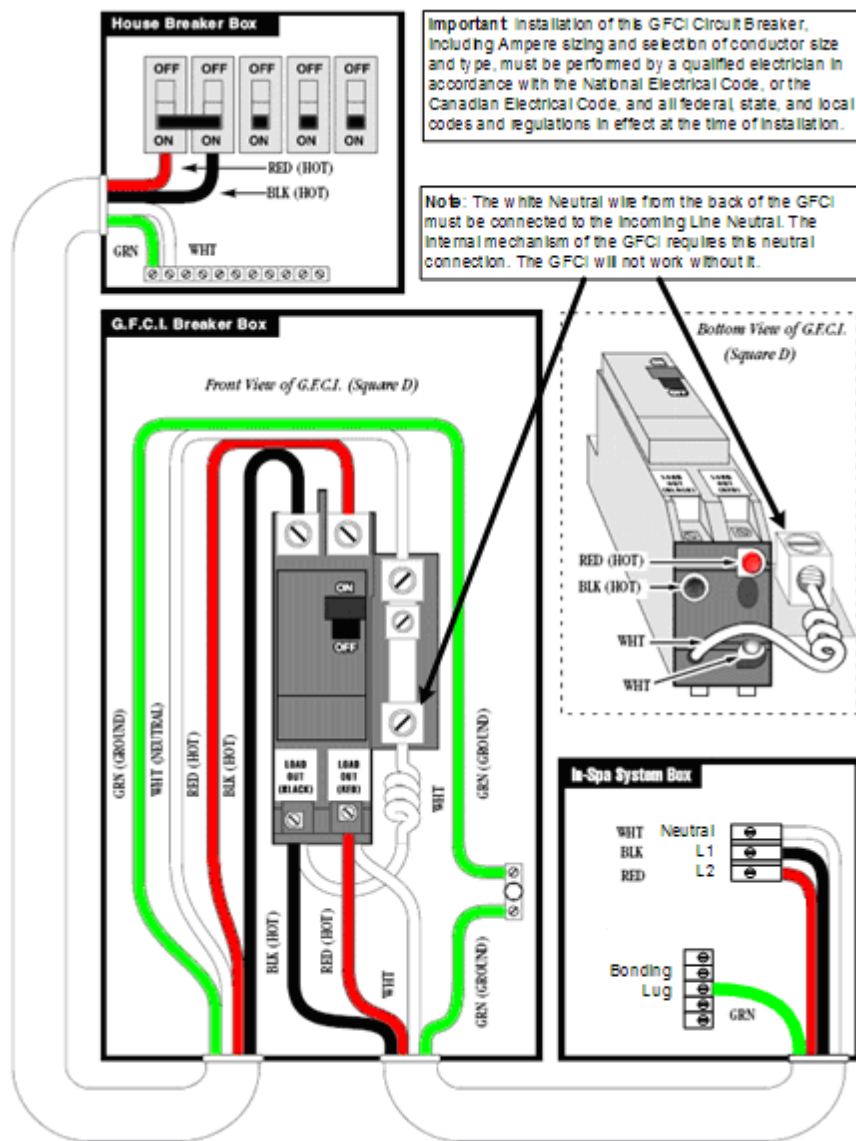
Figure 5 – US/Canada GFCI Diagram
