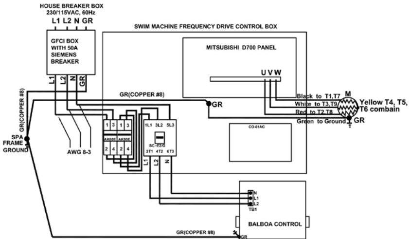
SWIMMER EDGE SE18 (US, CANADA). WIRING DIAGRAM FOR ONE POWER SERVICE (50A SIEMENS GFCI).
