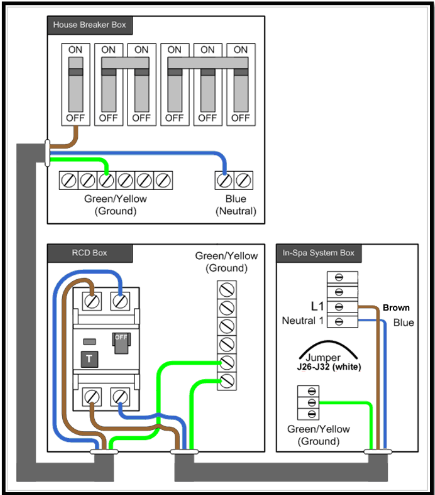
Figure 6 – Export 1x32A
