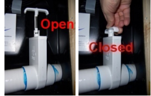
Figure 18 - Valve Open/Closed
