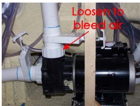
Figure 31 - Bleeding Air
