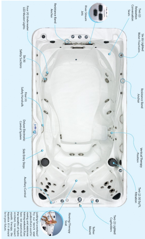
Figure 15 – Swim spa Callouts (AQ 14 Shown)
